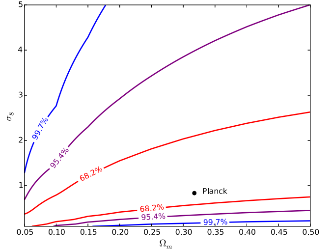
Figure 11. The likelihood-based confidence levels on \Omega_m and \sigma_8 , obtained from the 6dFGSv MV bulk flow measurement with R_1 = 70 h^{-1} Mpc. The black point indicates the best-fitting values found by Planck , used as the fiducial values in this work. The result for R_1 = 50 h^{-1} Mpc is very similar to this plot.
